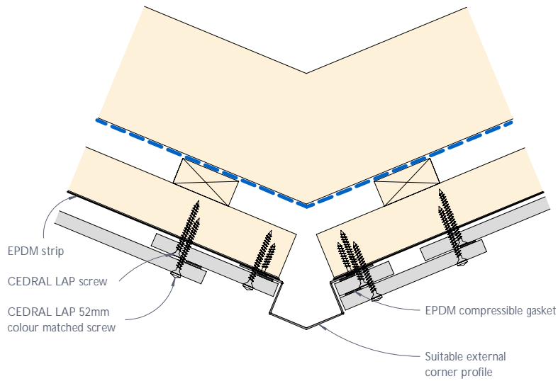
Figure 23: CEDRAL LAP 45 degree external corner
