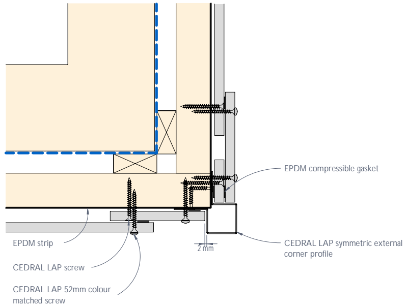
Figure 22: CEDRAL LAP typical external corner
